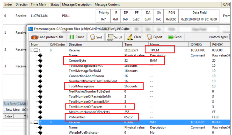
Figure 40. BAM message content.
