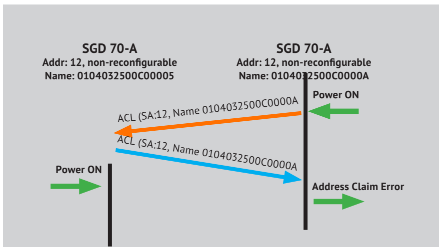
Figure 50. Multiple ECU Connection.
