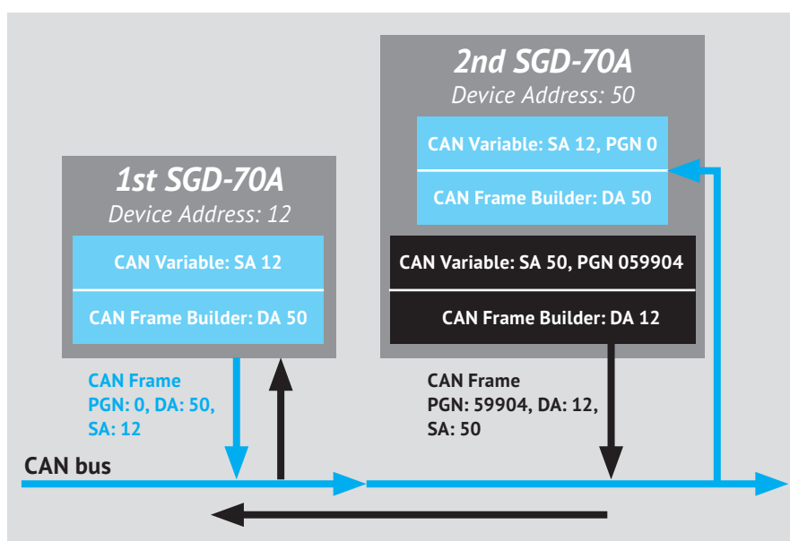
Figure 32. The Request PGN process.
